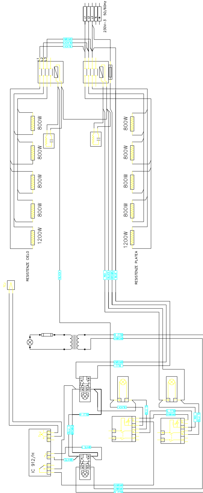
Figure 10-2. Electrical diagram for CIT 6 Modular at 230 Vac. 3 version.
