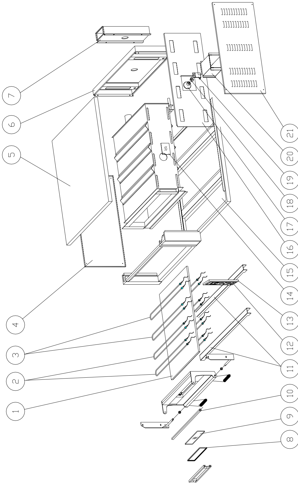
Figure 10-7 Exploded view
